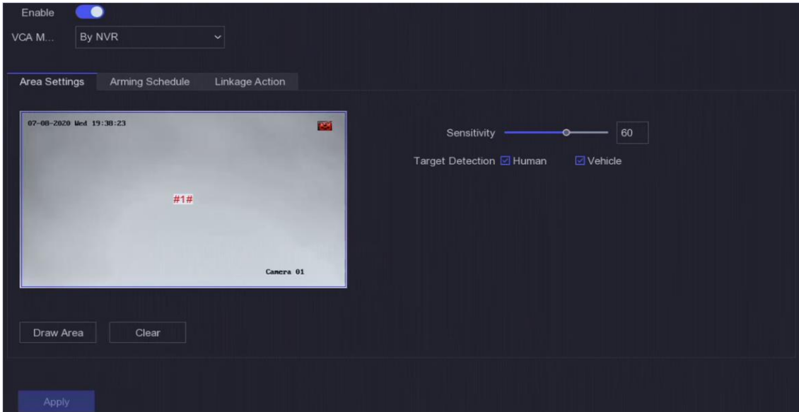
Figure 5-8 Motion Detection
