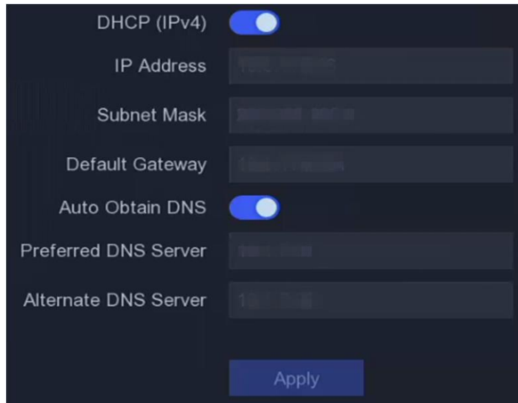
Figure 5-3 Network
