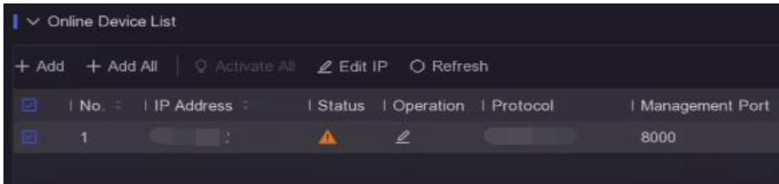
Figure 6-8 Online Device
