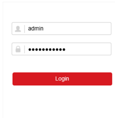
Figure 9-1 Login
