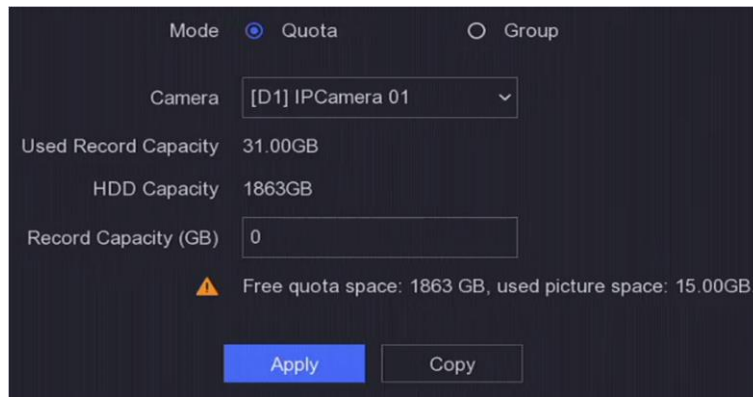
Figure 6-27 Quota
