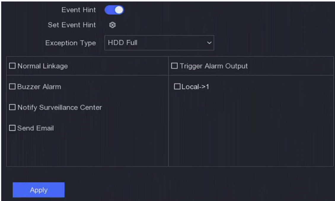
Figure 6-21 Exceptions
