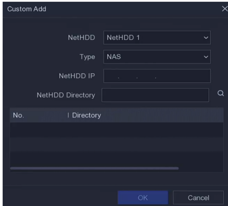
Figure 6-26 Add NetHDD
