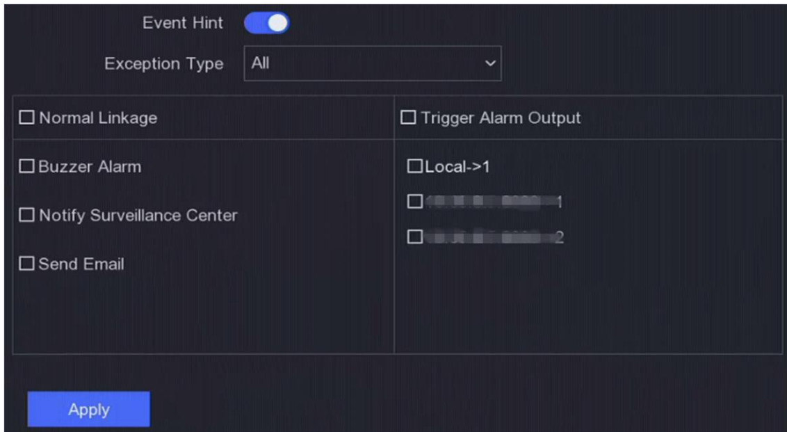
Figure 5-2 Exceptions
