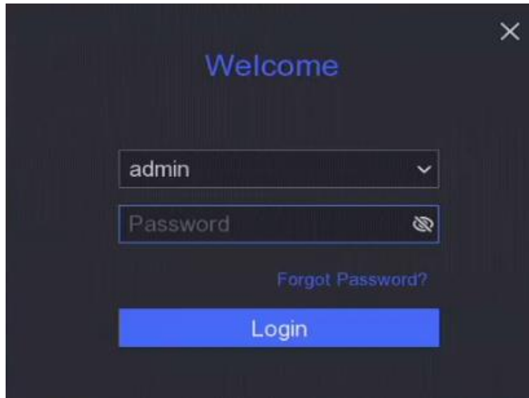
Figure 1-3 Login Interface
