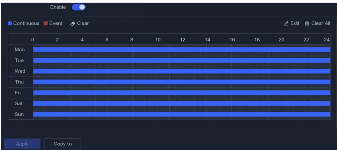
Figure 5-11 Recording Schedule
