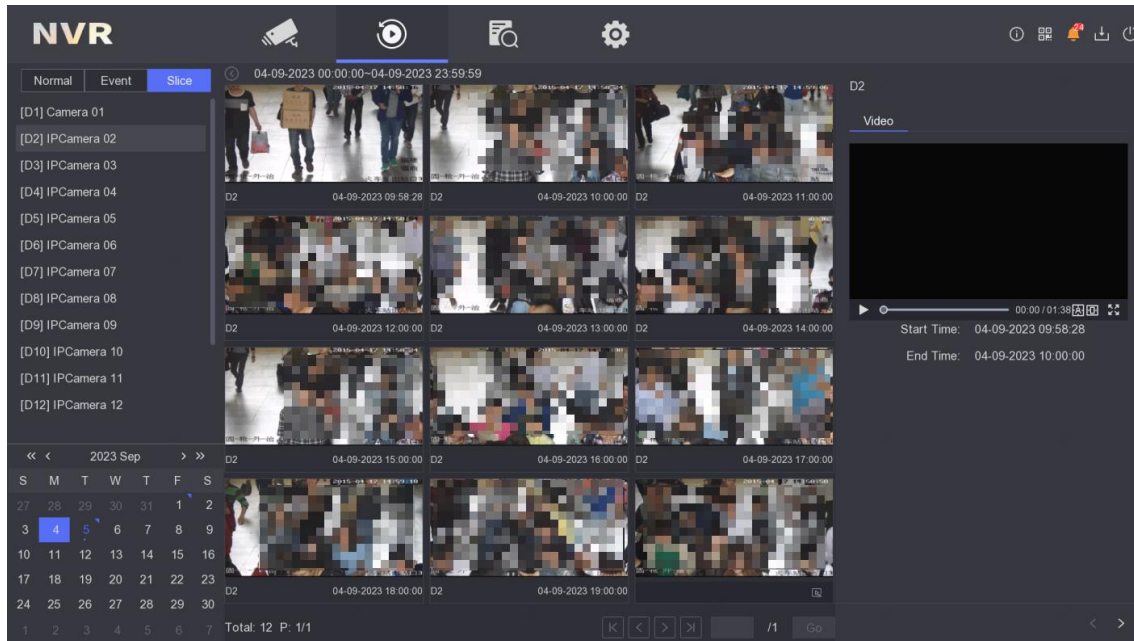
Figure 3-7 Video Slices
