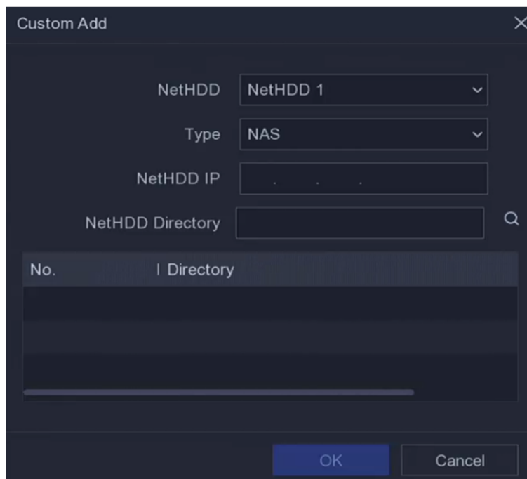
Figure 5-10 Add NetHDD
