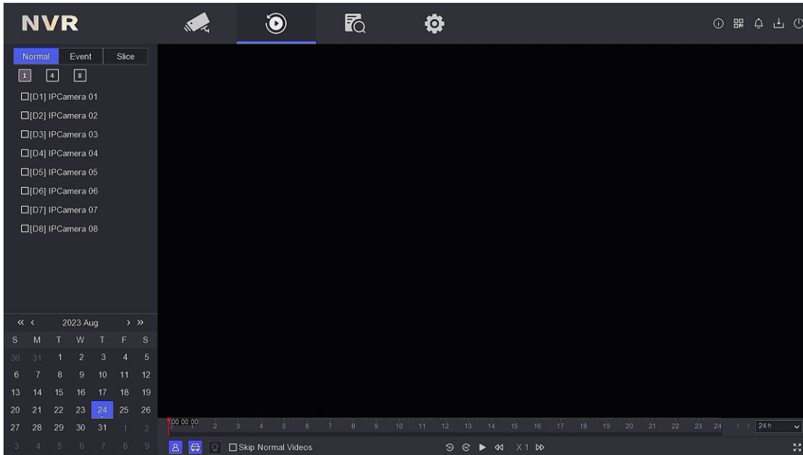
Figure 3-1 Playback
