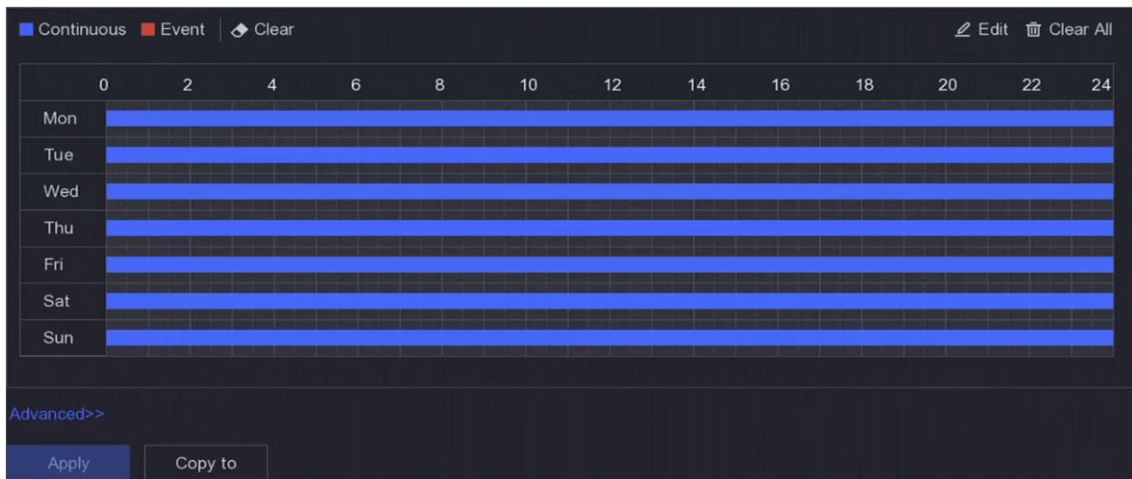
Figure 6-24 Recording Schedule
